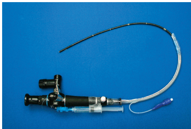
Fig. 1. Bronchoscope (Olympus PortaView® LF-GP Fiberscope) prepared with endotracheal tube and 20-gauge nylon closed-end multiorifice epidural catheter.
