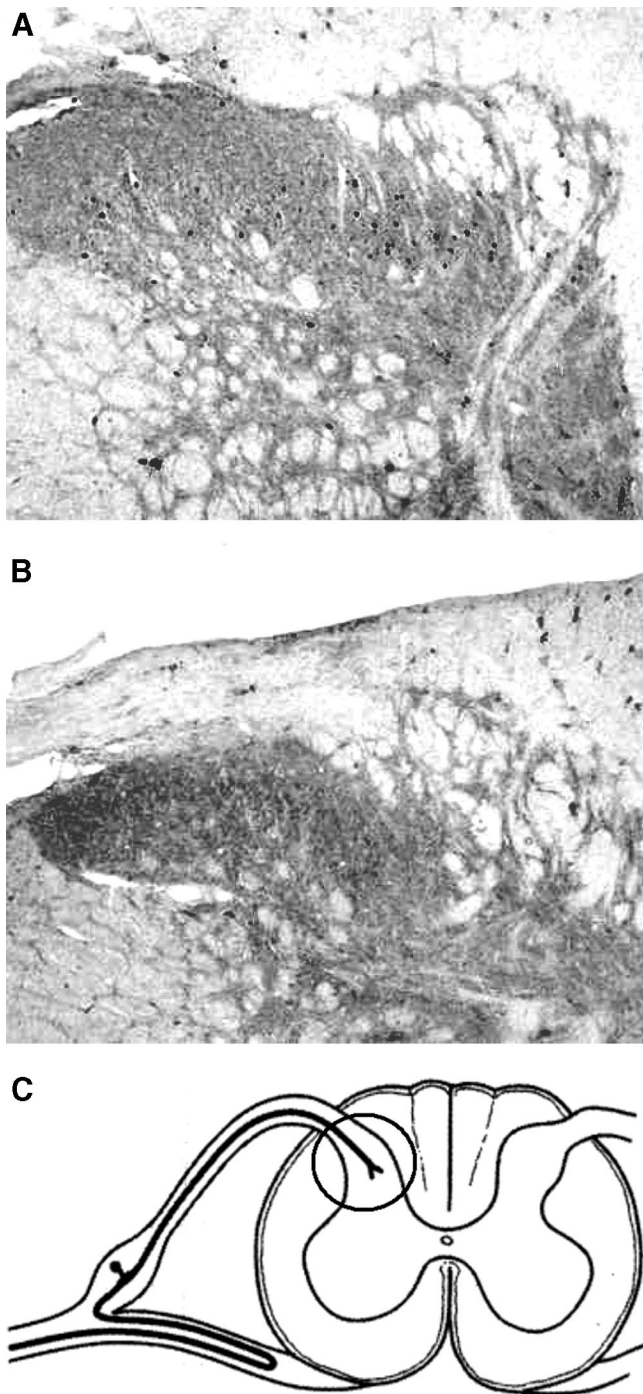
Fig. 1. Transverse sections of the cervical spinal cord at C5: nuclear c-Fos immunoreactive cells located in the dorsal horn of an animal treated with pulsed radiofrequency adjacent to the dorsal root ganglion (A) as compared with a sham operated animal (B). Schematic drawing of a transverse section of rat spinal cord at C5. The position of the area shown in A and B is indicated (C).
