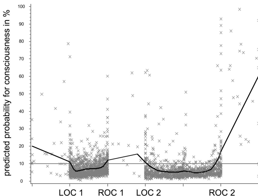
Fig. 3. Results of the best minimal model over time. The output value was calculated every 30 s from the start of the study until 10 min after loss of consciousness 2 (LOC 2) after the period of responsiveness, which includes loss of consciousness 1 at induction of anesthesia (LOC 1), and return of consciousness 1 after intubation (ROC 1). Additional data were from 10 min before return of consciousness 2 (ROC 2) until the end of the study. The 30-s interval was chosen because it corresponds with the clinical assessment of hypnosis, i.e. , the command "squeeze my hand." Lowess interpolation with smoothness factor 0.15 was applied for visualizing the classification through observation time. The best classification is reached with a cutoff value of 10% (horizontal line).
