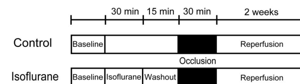
Fig. 1. Experimental protocols. (A) Two-hour reperfusion protocol. Mice were subjected to a 30-min coronary occlusion and 2 h of reperfusion. Isoflurane-treated mice received 1.0 minimum alveolar concentration of isoflurane followed by a memory period of 15 min before coronary occlusion. 5-Hydroxydecanoic acid (5-HD) or HMR-1098 was administered 55 min before occlusion. (B) Two-week reperfusion protocol. The mice were exposed to oxygen or isoflurane as described in the ischemia-reperfusion protocol and allowed to recover for 2 weeks.
