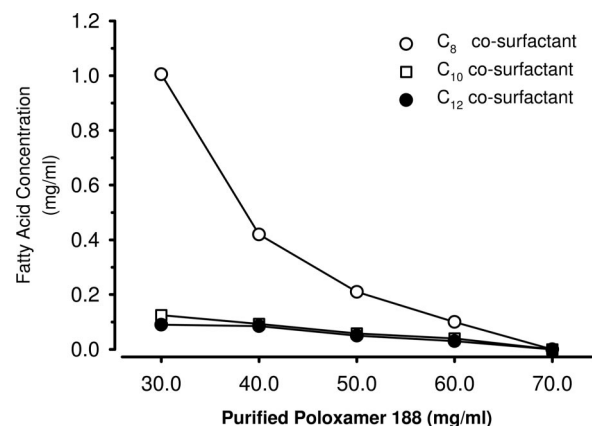
Fig. 3. Binary diagram noting the concentrations of purified poloxamer 188 and the cosurfactant fatty acids necessary to form propofol microemulsions in a bulk media of normal saline. The concentration of propofol was constant at 10 mg/ml. For a given fatty acid cosurfactant, the region below the line is a microemulsion, whereas the area above the line represents a macroemulsion formulation.
