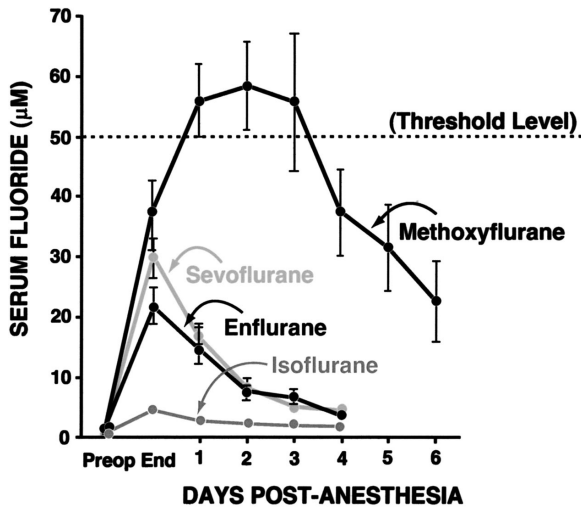
Fig. 2. Mean daily serum inorganic fluoride concentrations from patients anesthetized with methoxyflurane, 7 sevoflurane (data from the literature), 18 isoflurane, 18 and enflurane. 17 Patients anesthetized with methoxyflurane had higher serum inorganic fluoride concentrations that persisted longer than did those measured in the other subjects. Laboratory evidence of nephrotoxicity was seen at fluoride levels greater than 50 \mu\text{M} .
