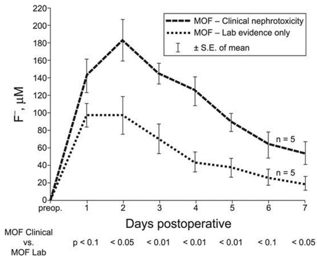
Fig. 1. Mean daily serum inorganic fluoride ( F^- ) concentrations. Patients anesthetized with methoxyflurane (MOF) were divided into two subgroups, those with laboratory abnormalities in renal function (MOF Lab; n = 5 ) and those with laboratory abnormalities as well as clinically evident renal dysfunction (MOF Clinical; n = 5 ). 1 Preoperative inorganic fluoride concentration was approximately 1 \mu M in all patients with no change after halothane anesthesia. Reprinted with permission from Mazze et al. 1
