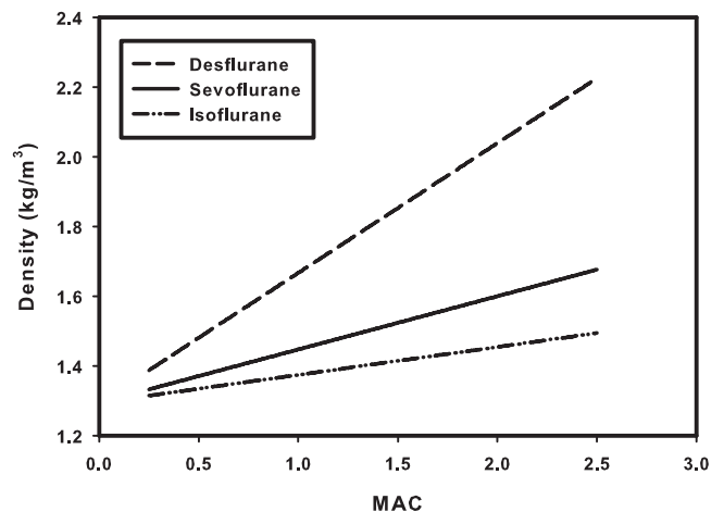
Fig. 1. Density at standard temperature and pressure (0°C and 1 atm) of admixtures of various minimal alveolar concentration (MAC)-multiples of isoflurane, sevoflurane, and desflurane in 25% oxygen and 75% nitrogen.
