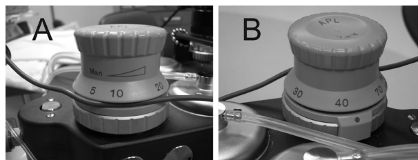
Fig. 1. (A) Rear view, recreated. Temperature cable trapped between knob and base of the automatic pressure limiting valve. (B) Front view, recreated. Automatic pressure limiting knob shields view of cable trapped beneath knob. Elevation of knob is subtle and easily missed.
