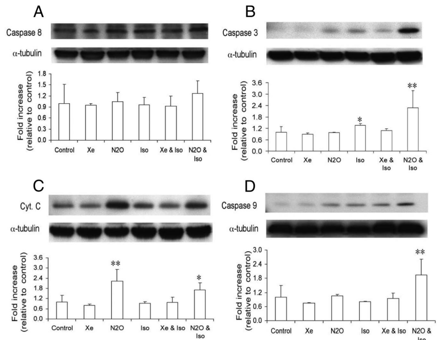
Fig. 3. Effects of anesthetic exposure (75% nitrous oxide [N 2 O], 75% xenon [Xe], 0.75% isoflurane [Iso], 0.75% Iso plus 75% N 2 O, or 0.75% Iso plus 60% Xe) for 6 h in day 7 rats on expression of signaling components of apoptotic pathways. Representative immunoblotting images and mean \pm SD (n = 4) of expression of caspase 8 (A), caspase 3 (B), cytosolic cytochrome c (C), and caspase 9 (D) induced by each anesthetic exposure as reflected by the band density normalized with \alpha -tubulin. Control = air exposure; Cyt. C = cytochrome c. * P < 0.05 , ** P < 0.01 versus control.
