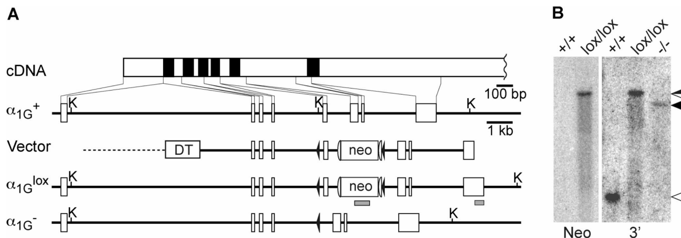
Fig. 1. Generation of \alpha_{1G} T-type calcium channel knockout mice by a Cre/loxP recombination system. (A) Schematic representation of \alpha_{1G} T-type calcium channel complementary DNA (cDNA), \alpha_{1G}^+ allele ( \alpha_{1G}^+ ), targeting vector (Vector), targeted \alpha_{1G}^{\text{lox}} allele ( \alpha_{1G}^{\text{lox}} ), and \alpha_{1G}^- allele ( \alpha_{1G}^- ) after Cre-mediated recombination. Black areas of cDNA represent the nucleotide sequences encoding the membrane spanning segments S1–S6 of repeat I of the \alpha_{1G} channel. White boxes represent exon sequences, Pkg-1 promoter-neo-pA cassette (neo), and diphtheria toxin cassette (DT). LoxP and frt sites are shown by black triangles and white half-circles , respectively. Gray boxes indicate probe regions (neo and 3') used for Southern blot analysis. K is the KpnI site. (B) Southern blot analysis of genomic DNA from \alpha_{1G}^{+/+} , \alpha_{1G}^{\text{lox/lox}} , and \alpha_{1G}^{-/-} mice. Left: KpnI -digested DNA hybridized with a neo probe. Right: KpnI -digested DNA hybridized with a 3' probe. The black triangle indicates the 14.7-kb fragment from the \alpha_{1G}^- allele. The white triangle indicates the 5.9-kb fragment from the \alpha_{1G}^+ allele. The triangle with a black upper half indicates the 17.2-kb fragment from the \alpha_{1G}^{\text{lox}} allele.
