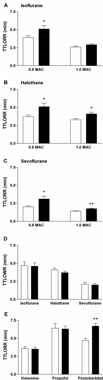
Fig. 2. Effects of volatile (A–D) and intravenous (E) anesthetics on time to loss of righting reflex (TTLORR) and time to loss of tail withdrawal reflex (TTLOWR) in wild-type (white bars) and mutant (black bars) mice. Values are mean \pm SEM ( n = 10 – 24 /group for volatile and n = 11 – 15 /group for intravenous anesthetics). * P < 0.05 , ** P < 0.01 , wild-type versus mutant mice. MAC = minimum alveolar concentration.
