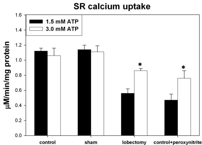
Fig. 4. Effect of doubling adenosine triphosphate (ATP) concentration on sarcoplasmic endorecticular calcium adenosine triphosphatase subtype 2a-mediated uptake of calcium by isolated sarcoplasmic reticulum (SR) vesicles. For control and sham samples, increased ATP had no effect on calcium uptake. In contrast, higher ATP concentration significantly increased SR calcium uptake in samples from lobectomy animals and from control samples pretreated with 100 \mu M peroxynitrite. * Difference between 1.5 mM and 3.0 mM ATP.
