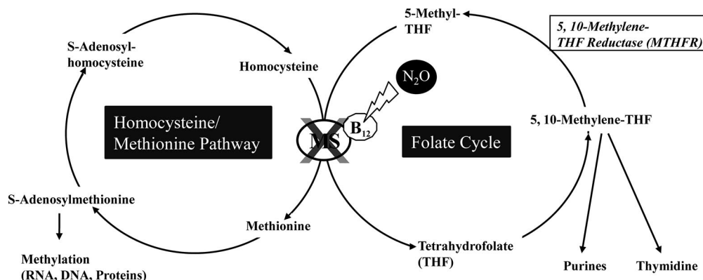
Fig. 1. Inhibition of methionine synthase (MS) by nitrous oxide ( N_2O ) occurs at a critical juncture of two pathways: the folate cycle and the remethylation of methionine from homocysteine. Nitrous oxide oxidizes the cobalt atom of vitamin B_{12} (cobalamin), thereby inactivating vitamin B_{12} as a necessary cofactor for methionine synthase function. The subsequent accumulation of 5-methyl-tetrahydrofolate due to inactive methionine synthase is called "folate trapping." THF = tetrahydrofolate.
