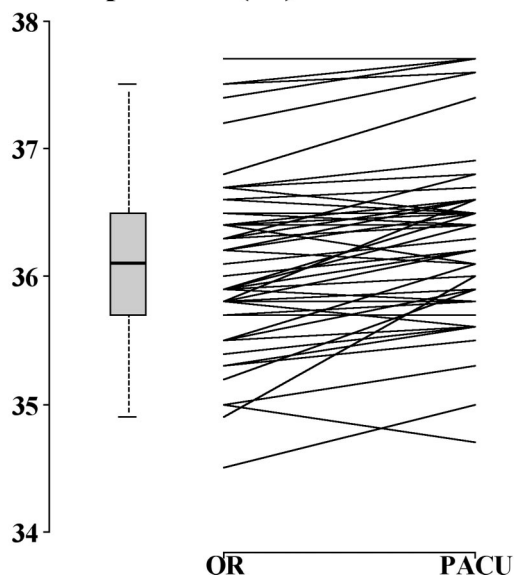
Fig. 1. Individual changes in bladder temperature from the operating room (OR) at the end of surgery until arrival in the postanesthesia care unit (PACU). Box plots of the final measurement in the OR and temperature upon arrival in the PACU. The middle, upper edge, and the lower edge of the box indicate the 50 th , 75 th , and 25 th percentile of the data set. The ends of the vertical lines indicate 1.5 times the interquartile range. The difference averaged 0.2 \pm 0.3^{\circ}\text{C} (95% confidence interval 0.13 to 0.29^{\circ}\text{C} ), P < 0.001 . The average time elapsed between removal of the esophageal stethoscope and arrival in the PACU was 30 \pm 12 min.
