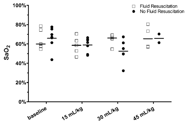
Fig. 4. Arterial hemoglobin oxygen saturation ( SaO_2 ) measured at peripheral oxygen saturation ( SpO_2 ) less than 70% at different levels of hemorrhage. Arterial blood gases were taken when SpO_2 reached 70%. Fluid resuscitated (□) versus non-fluid-resuscitated (●) animals.
