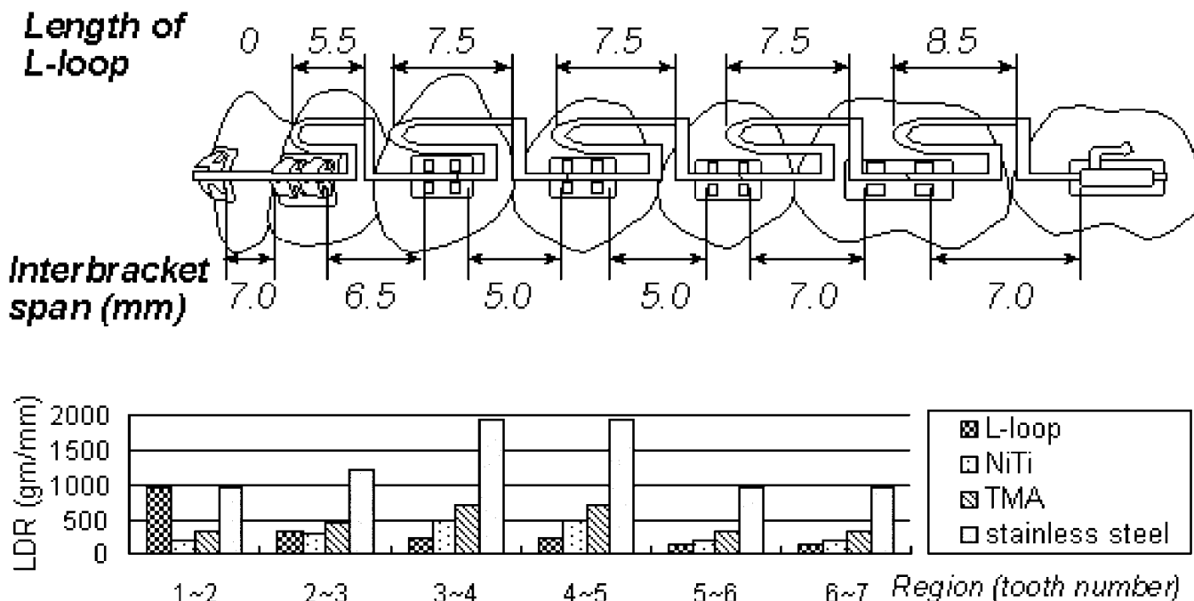
FIGURE 5. The load deflection rate in each interbracket span (maxilla).
