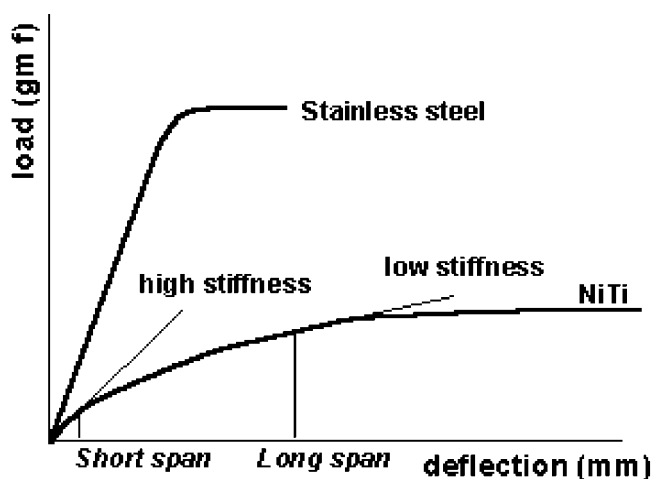
FIGURE 7. Load-deflection curve of stainless steel and nickel-titanium wires.
