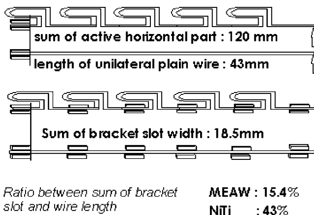
FIGURE 8. Ratio between the sum of bracket and wire length.
