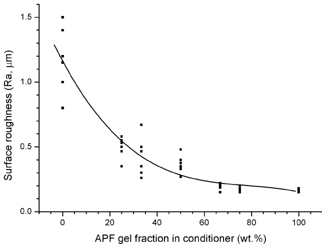
FIGURE 3. Surface roughness as function of the acidulated phosphate fluoride (APF) fraction on etchant.
