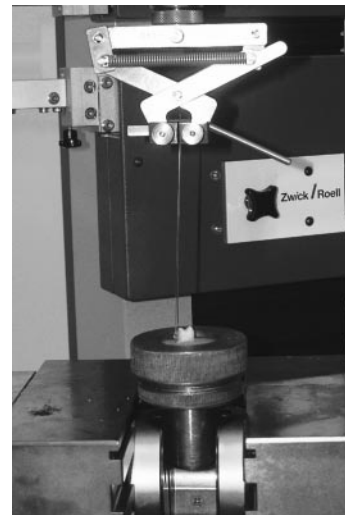
FIGURE 1. Specimen in Zwick Universal Test machine.
