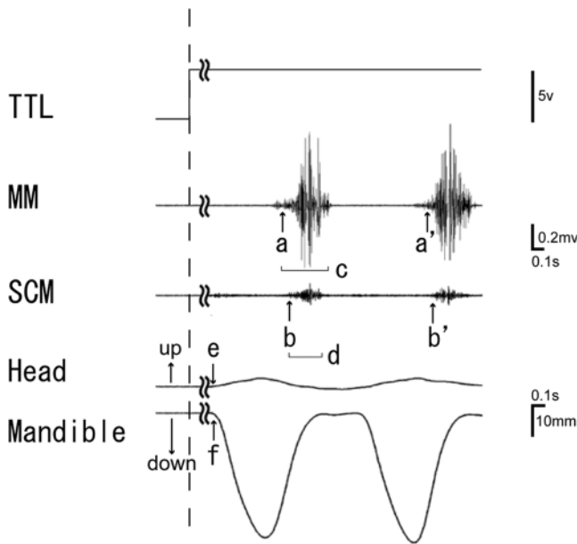
FIGURE 2. An Example of measurement data and the analytic factors. A vertical axis is TTL: TTL (Transistor Transistor Logic) level; MM: right MM activity; SCM: right SCM activity; Head: head movement in relation to the head sequentially from the top. Horizontal axis is time. a: MM activity onset; b: SCM activity onset; c: time of MM activity; d: time of SCM activity; e: start point of head movement; f: start point of mandibular movement; a'-a: MM activity cycle; b'-b: SCM activity cycle; f'-f: mandibular movement cycle; e'-e: head movement cycle; f-e: onset difference between head movement to mandibular movement; b-a: the onset difference between the MM activity and SCM activity; D : 3-dimensional distance of mandibular and head movement [ D = \sum_{t=1}^n \sqrt{(x_t - x_{t-1})^2 + (y_t - y_{t-1})^2 + (z_t - z_{t-1})^2} ( x : right and left direction; y : forward and backward direction; z : upward and downward direction)].
