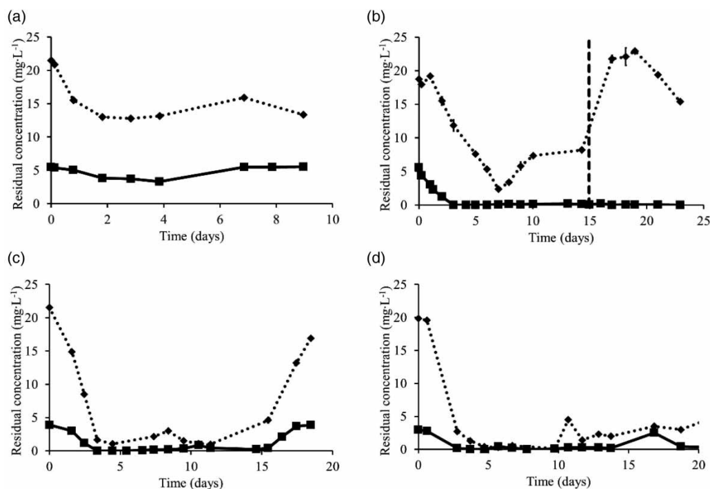
Figure 3 | Ammonium and nitrate remediation for site A samples for (a) 3 h, (b) 6 h (addition of fresh feed on day 15.0), (c) 12 h and (d) 20 h HRT. NH 4 -N (■) and NO 3 -N (◆). Average influent concentration 4.2 mg·L -1 NH 4 -N and 20.3 mg·L -1 NO 3 -N.
