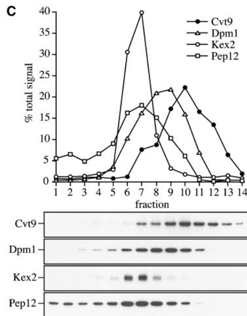
Figure 4. Cvt9 is localized to a perivacuolar compartment. (A) Localization pattern of GFPCvt9. The cvt9Δ (AHY001) strain was transformed with a plasmid encoding a GFPCvt9 fusion protein behind the CUP1 promoter (pCuGFPCVT9). Expression of GFPCvt9 was induced with 10 \mu M CuSO 4 for 2 h, followed by labeling of the vacuoles with FM 4-64 (see Materials and Methods). Images were taken with a Leica IRM confocal microscope. GFPCvt9 mostly localizes to intense perivacuolar, punctate structures. (B and C) Subcellular localization of Cvt9 by Optiprep density gradients. The cvt9Δ strain was transformed with
