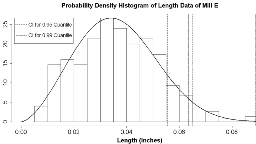
Figure 5.—Histogram and density function plot for Mill E (no censoring) with bootstrap confidence intervals for the 0.95 and 0.99 quantiles.
