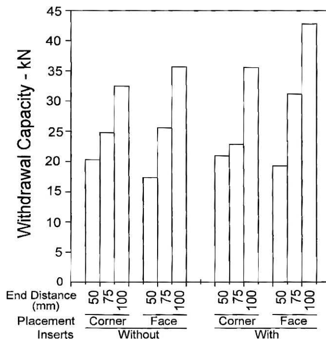
Figure 7.—Withdrawal capacity of 15.9-mm (nominal 5/8-in.) through-bolts with 25-mm (nominal 1-in.) pipe-nuts in nominal 89 by 89-mm (nominal 3½ by 3½-in.) western hemlock members.
