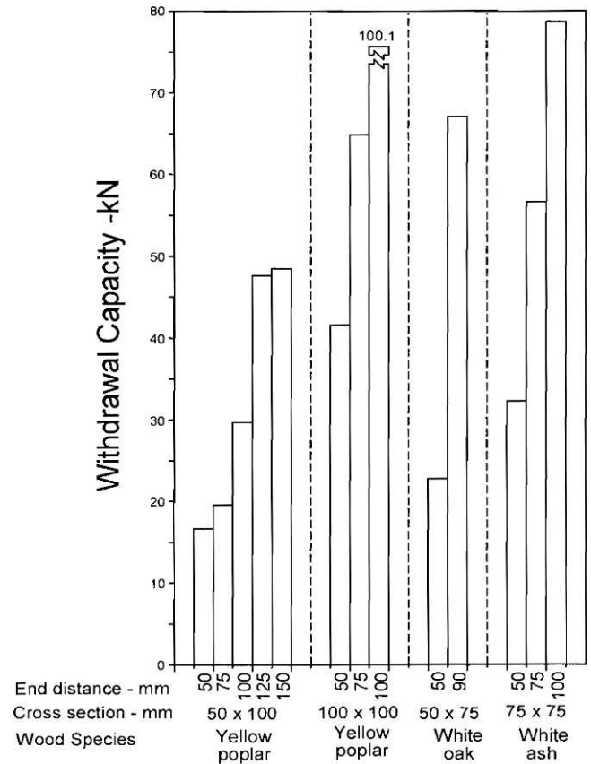
Figure 9.—Withdrawal capacities of 15.9-mm (nominal 5/8-in.) through-bolts with 25-mm (nominal 1-in.) pipe-nuts with inserts in yellow poplar, white oak, and white ash members.
