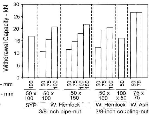
Figure 10.—Withdrawal capacities of 9.5-mm (nominal 3/8-in.) through-bolts and 15-mm (nominal 1/2-in.) pipe-nuts and of 9.5-mm through-bolts and 10-mm (nominal 3/8-in.) pipe-coupling-nuts in southern yellow pine (SYP), western hemlock, and white ash.
