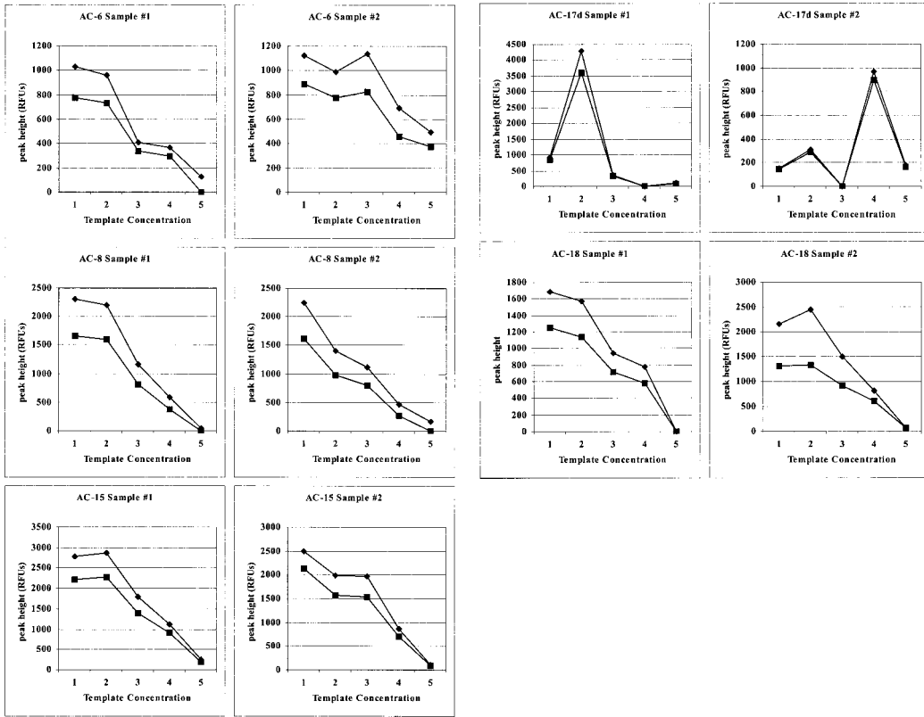
Figure 1. Fluorescent signal of alligator microsatellite alleles using 10-fold serially diluted alligator DNA as template. Sample 1 concentration 1 was 135 ng/μl, sample 2 concentration 1 was 170 ng/μl. All loci are heterozygous. The shorter allele is plotted with diamonds.
