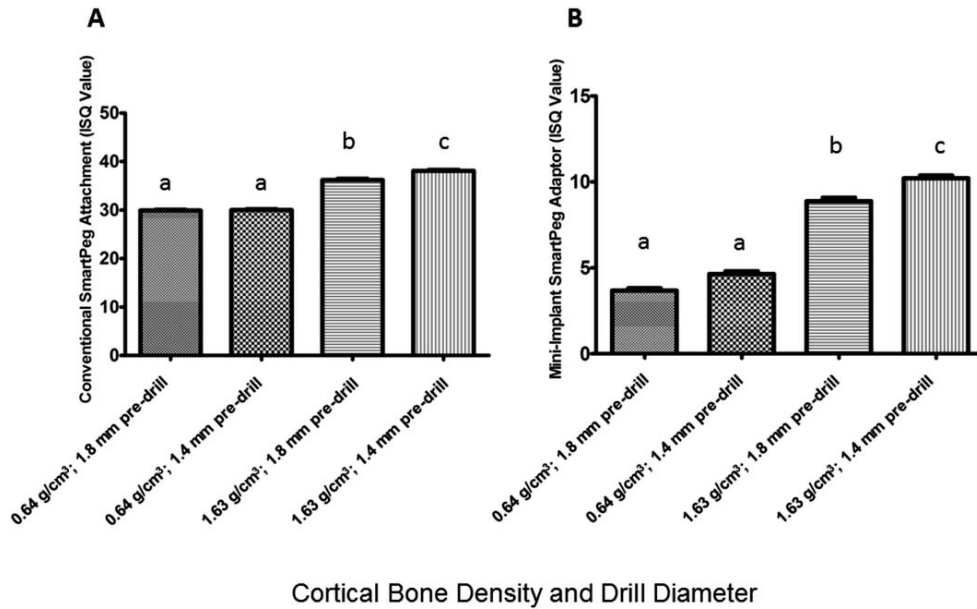
Figure 4. ISQ measurements for the various stability levels obtained using conventional SmartPeg attachment (A) and the MISPA (B). Bars represent means ± SEM, n = 180 ISQ values per group (15 mini-implants per group × 4 ISQ measurements per implant × 3 test days). Kruskal-Wallis tests detected similar differences ( P < .0001 ) among the various stability levels for both attachment techniques. Dunn’s multiple-comparison tests were used to assess differences between groups; different lowercase letters indicate significant differences between groups ( P < .05 ).
