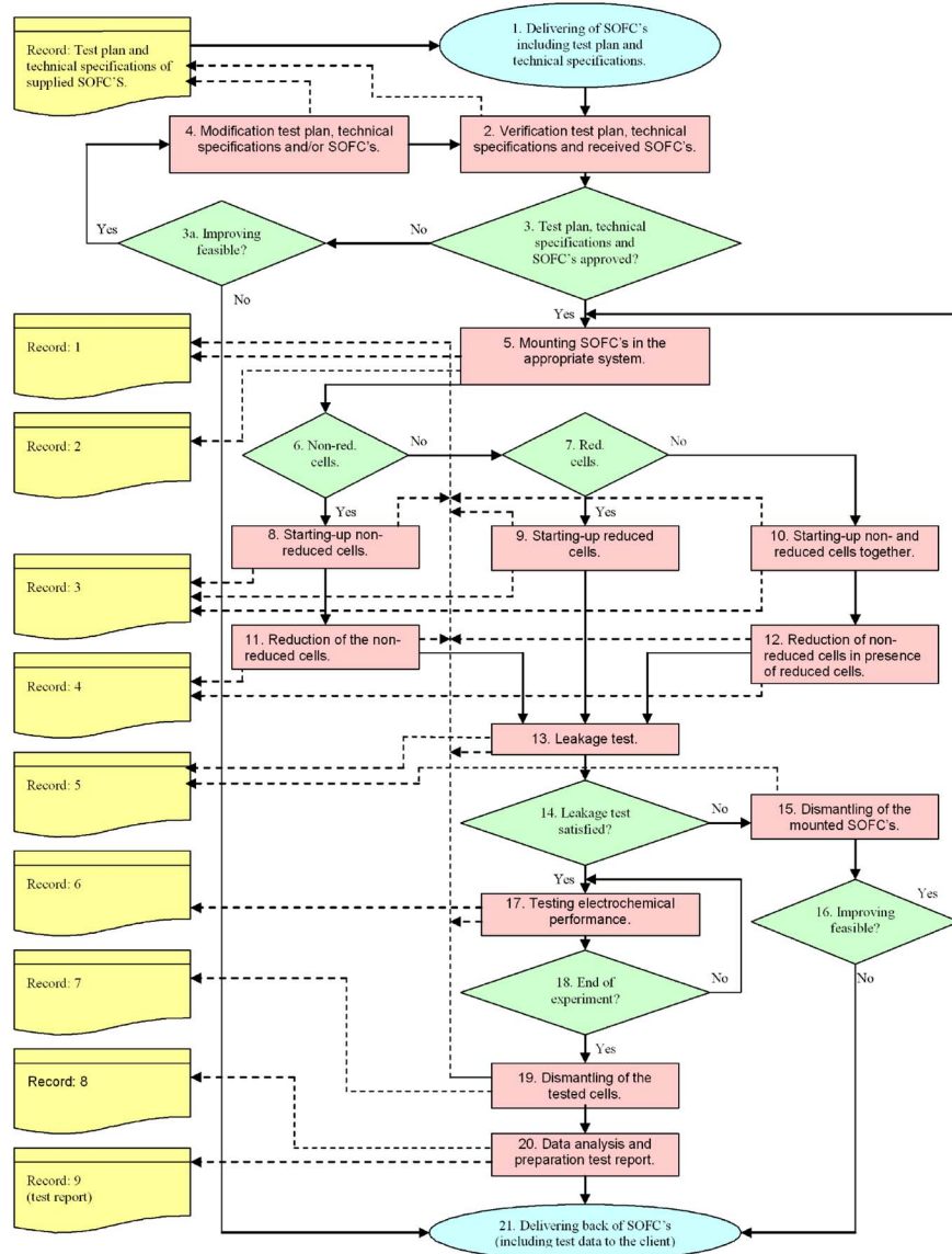
Fig. 2 Flowchart of testing procedure for single cells at FZJ
