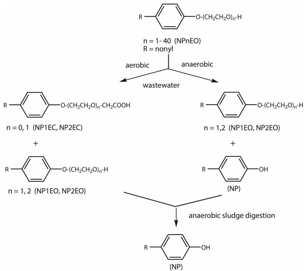
Fig. 1. Aerobic and anaerobic degradation of NPE; modified from Ahel et al. (1994a).
