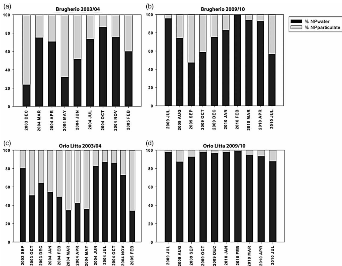
Fig. 6. Percentage of NP dissolved in water vs percentage adsorbed to SPM in two sampling campaigns, in two sample sites: (a) Brugherio (S2) 2003/04, (b) Brugherio (S2) 2009/10, (c) Orio Litta (S3) 2003/04, (d) Orio Litta (S3) 2009/10.
