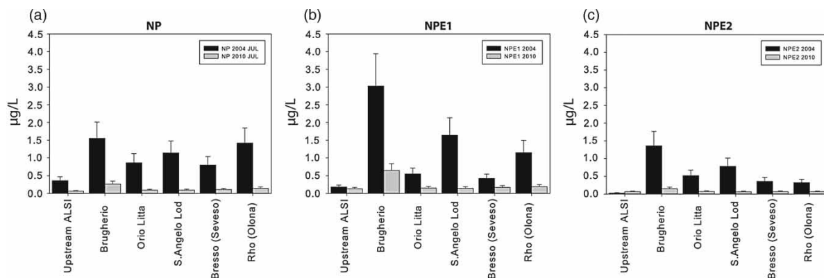
Fig. 5. Concentrations of NP (a), NPE1 (b) and NPE2 (c) measured in the two different years (2004 July and 2010 July) in six sampling stations: Upstream ALSI (S1), Brugherio (S2), Orio Litta (S3), S. Angelo Lodigiano (S4), Bresso (S5), Rho (S6). Bars are one standard deviation ( n = 3 ).
