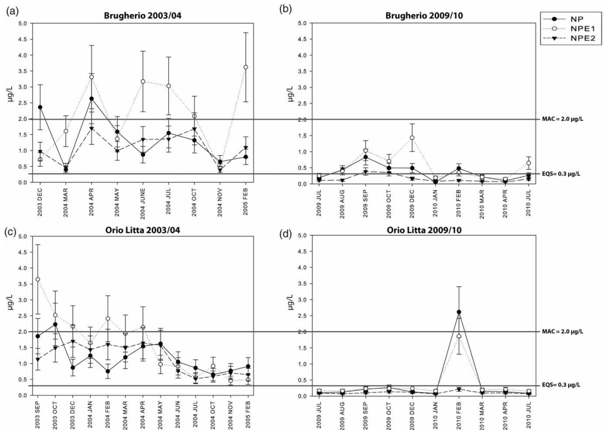
Fig. 3. NP, NPE1 and NPE2 concentrations measured in two sampling campaigns, in two sample sites: (a) Brugherio (S2) 2003/04, (b) Brugherio (S2) 2009/10, (c) Orio Litta (S3) 2003/04, (d) Orio Litta (S3) 2009/10. Bars are one standard deviation ( n = 3 ).
