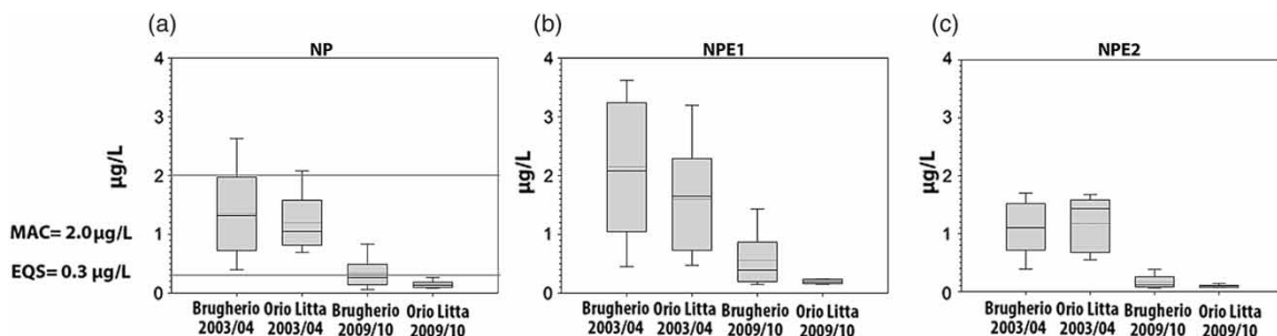
Fig. 4. NP (a), NPE1 (b) and NPE2 (c) concentrations in two sampling campaigns, in two sample sites (Brugherio (S2) 2003/04, Orio Litta (S3) 2003/04, Brugherio (S2) 2009/10, Orio Litta (S3) 2009/10). Vertical boxes represent 25th and 75th percentiles, whiskers are at 10th and 90th percentiles, median (continuous line) and mean (dotted line) values. (a) Mean values for NP are, respectively, from left to right 1.35 \mu\text{g/L} , 1.20 \mu\text{g/L} , 0.34 \mu\text{g/L} , 0.15 \mu\text{g/L} .
