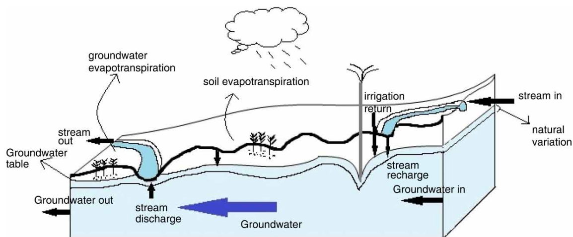
Fig. 4. The conceptual model.
