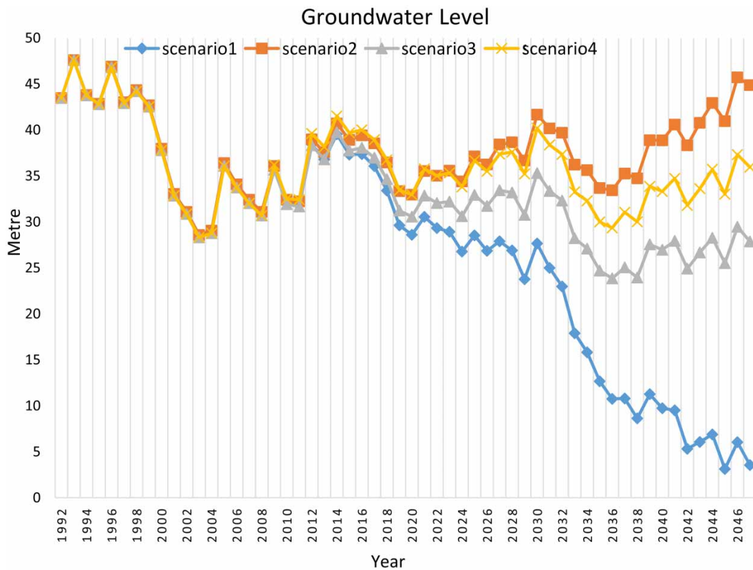
Fig. 14. Groundwater level, different scenarios.
