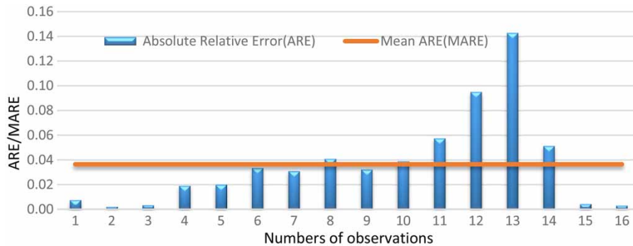
Fig. 12. Absolute relative error (ARE) and mean absolute relative error (MARE).
