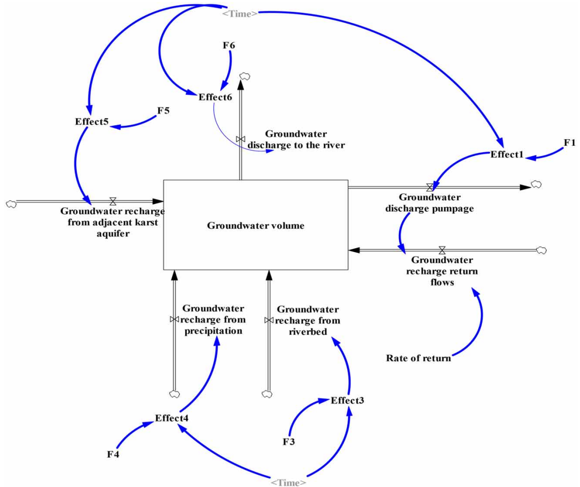
Fig. 7. Groundwater volume, inflow and outflow.
