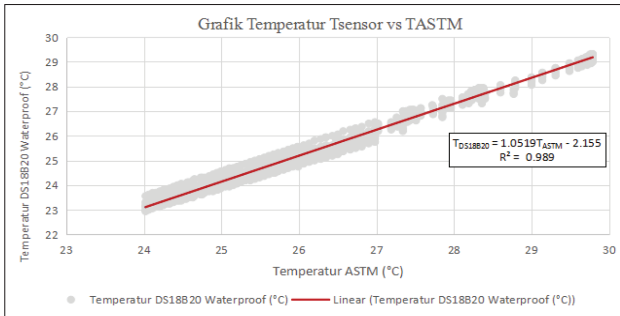
FIGURE 3. Linear Regression
