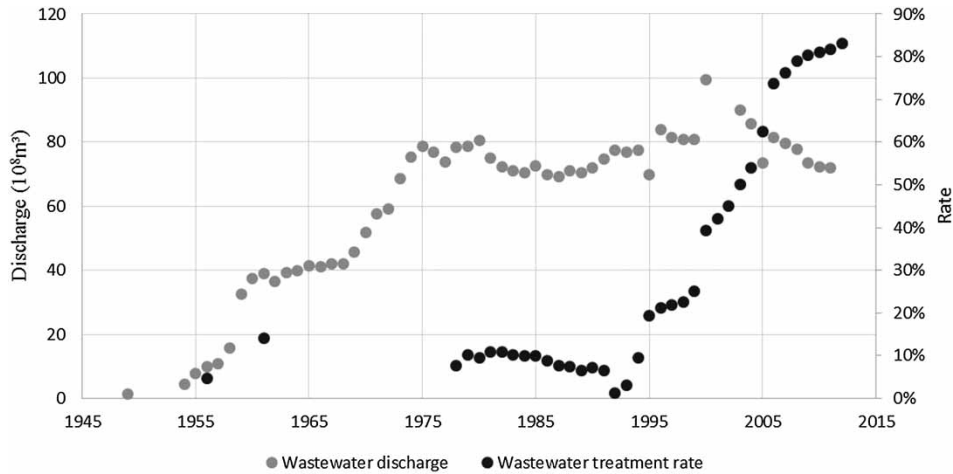
Fig. 8. Volume of Beijing wastewater discharge and treatment rate. Unit: (10 8 m 3 ).
