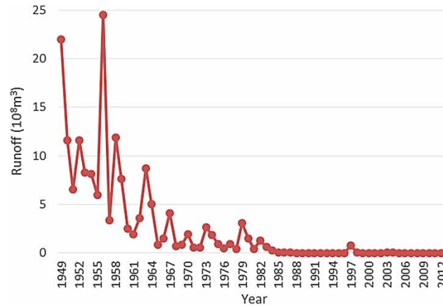
Fig. 6. The evolution of the Yongding River runoff (Sanjiadian Hydrological Station). Unit: ( 10^8 \text{ m}^3 ).
