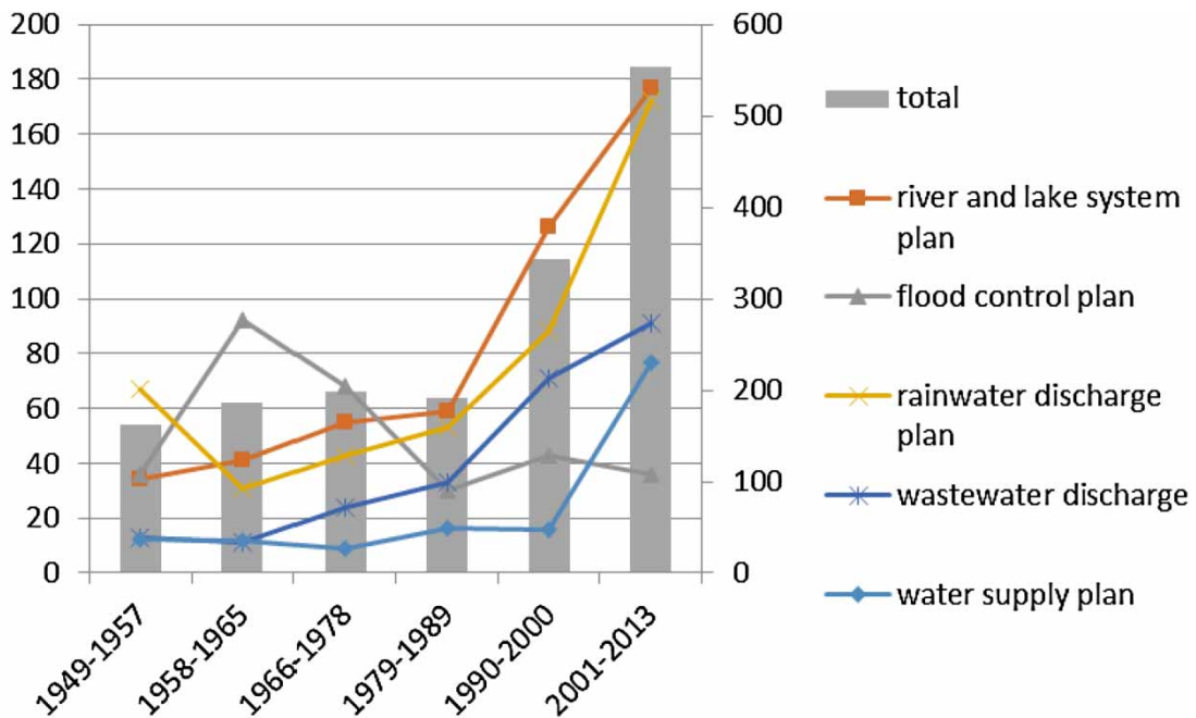
Fig. 3. Frequencies of five planning categories in six temporal stages.
