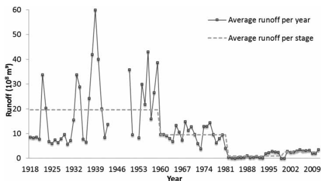
Fig. 5. The evolution of the Chaobai River runoff (Suzhuang Hydrological Station). Unit: ( 10^8 \text{ m}^3 ).
