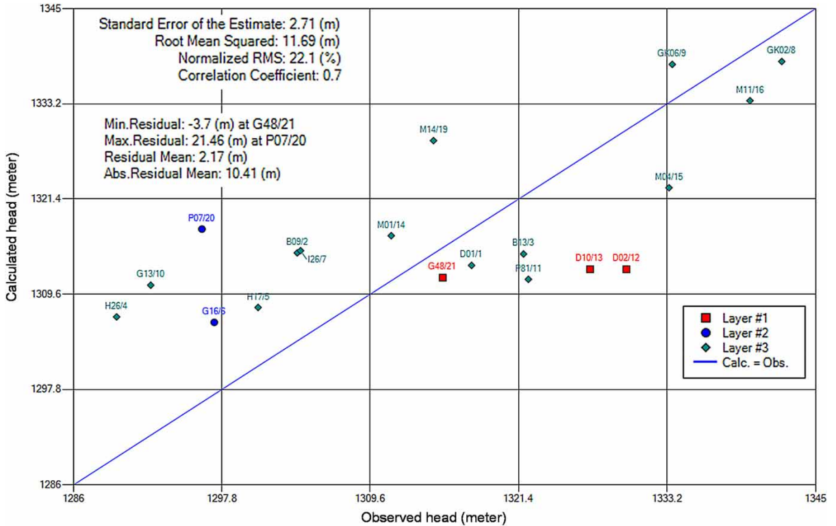
Fig. 5. Calibration of hydraulic heads for January 2003 using unpublished observed values from GWRDB (Groundwater Resources Development Board).
