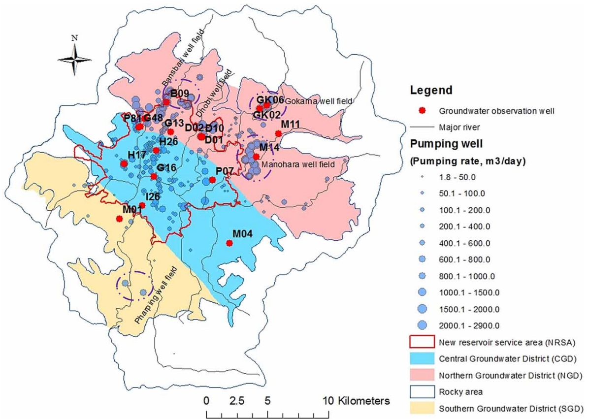
Fig. 4. Spatial distribution of pumping wells with abstraction rates at northern, central, and southern groundwater districts of the Kathmandu Valley.
