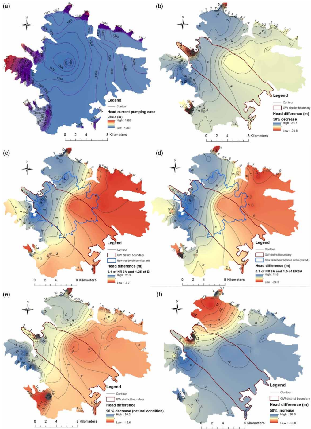
Fig. 7. Simulated heads in the baseline scenario (a) and head changes between the baseline and (b) 50% reduction, (c) minimal (10%) in the new RSA and 25% increase in the existing RSA, (d) minimal (10%) in the new RCA and 50% increase in the existing RSA, (e) optimistic, and (f) pessimistic scenarios.
