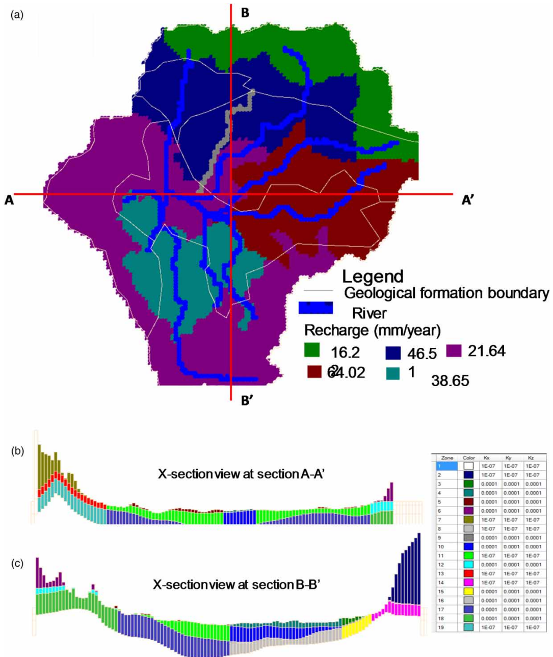
Fig. 3. Groundwater flow model setup in the Visual MODFLOW Flex for Kathmandu Valley: (a) top view of aquifer recharge zones with river and drain networks and boundary of reclassified geologic formations utilized for property zones. Cross sections with hydraulic conductivity zone values are shown in (b) A–A' and (c) B–B'.
