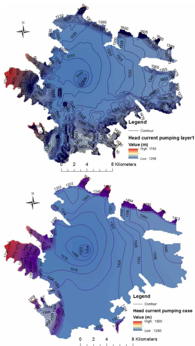
Fig. 6. Spatial distribution of simulated hydraulic heads in the shallow (top) and deep (bottom) aquifers in the three groundwater districts within the Kathmandu Valley using the calibrated model. Head values are in meters above mean sea level.
