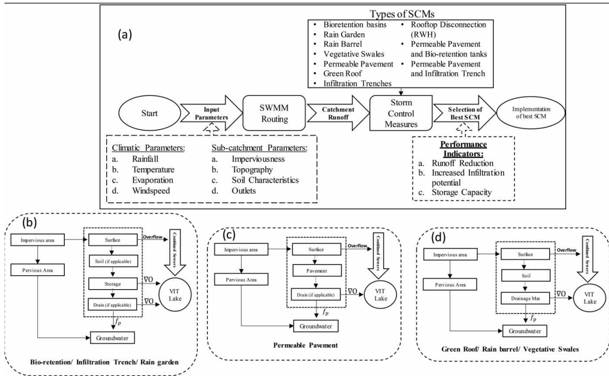
Fig. 2. (a) Detailed methodology flowchart; (b) storage type SCMs; (c) bypass type SCMs and (d) combination of by-pass and storage type SCMs.
