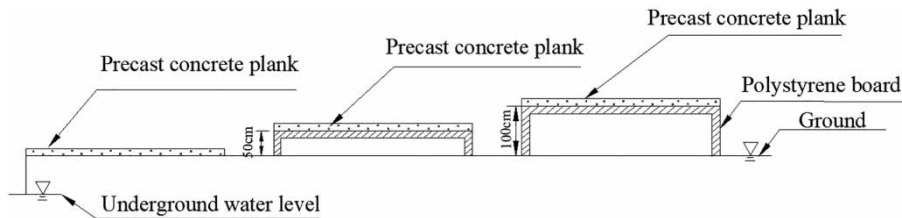
Fig. 3. Profile plan of the different groundwater platforms.
