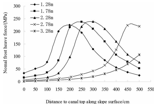
Fig. 8. Distribution of the normal frost heave force of the canal slope with the different groundwater levels.
