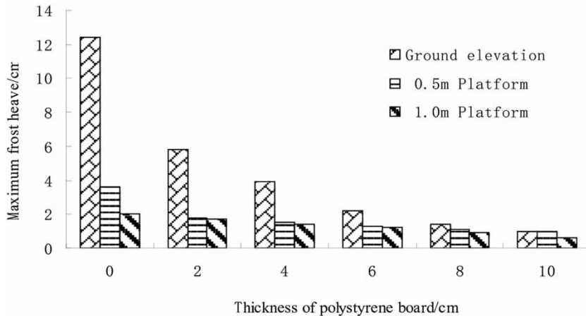
Fig. 6. Maximum frost heave of the EPS plates with different thicknesses.
