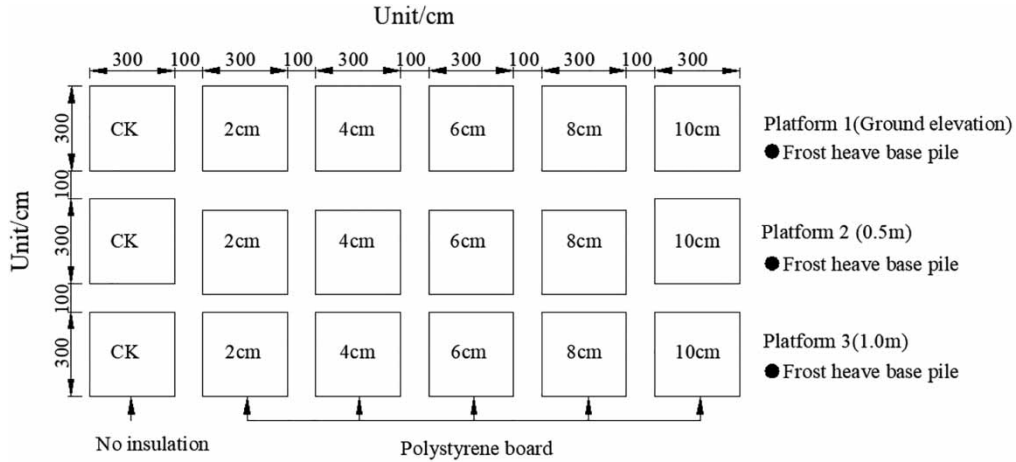
Fig. 2. Floor plan of the different groundwater platforms.
