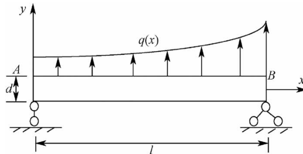
Fig. 7. Distribution of the normal frost heaving force on the lining plate.
