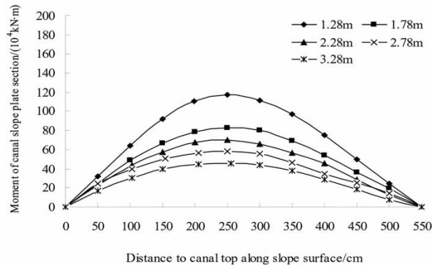
Fig. 9. Section bending moment diagram of the canal slope plate under the different groundwater depths.
