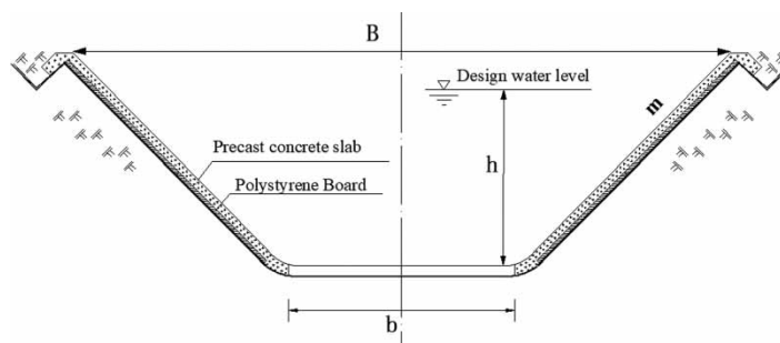
Fig. 4. Typical channel profile (B, top width; b, floor width; h, design water level buried depth; m, slope ratio).
