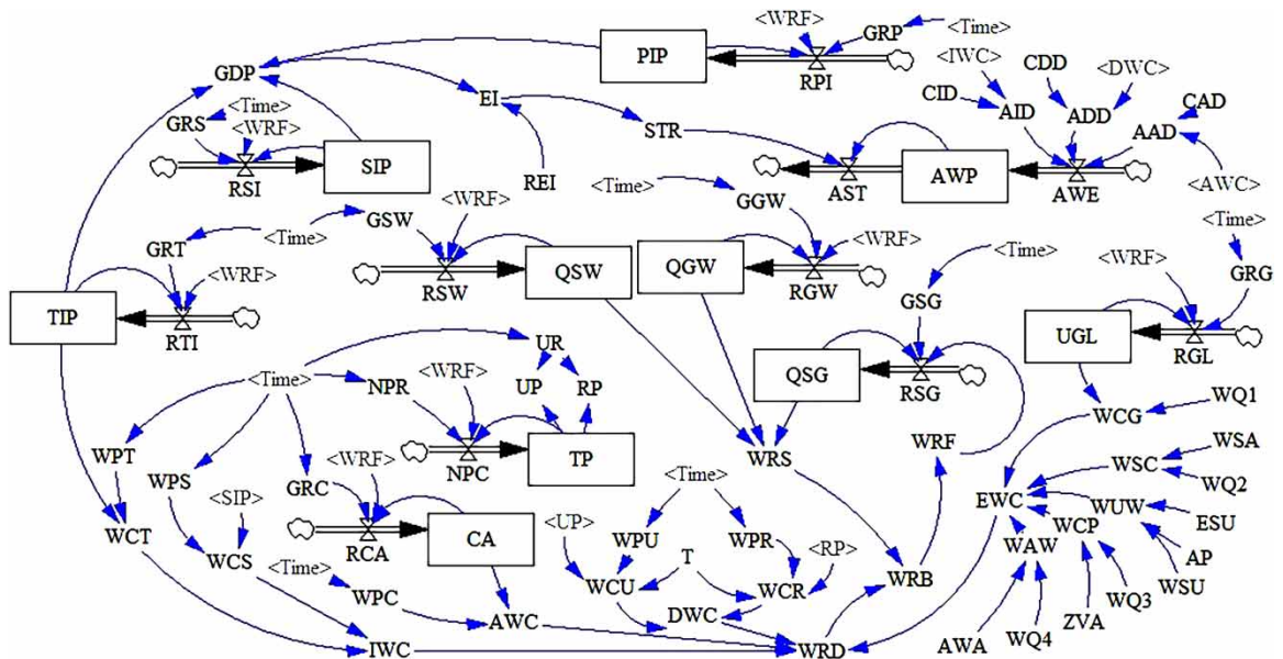
Fig. 2. Stocks and flows of the simulated system.
