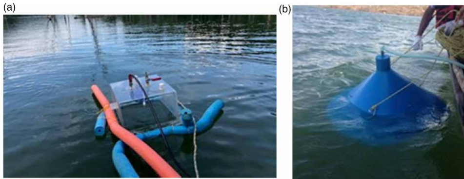
Fig. 2 | GHG monitoring: (a) floating static chamber scheme for monitoring diffusive flows and (b) inverted funnel for bubbling gases.
