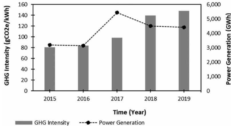
Fig. 4 | The relationship between GHG intensity and power generation.
