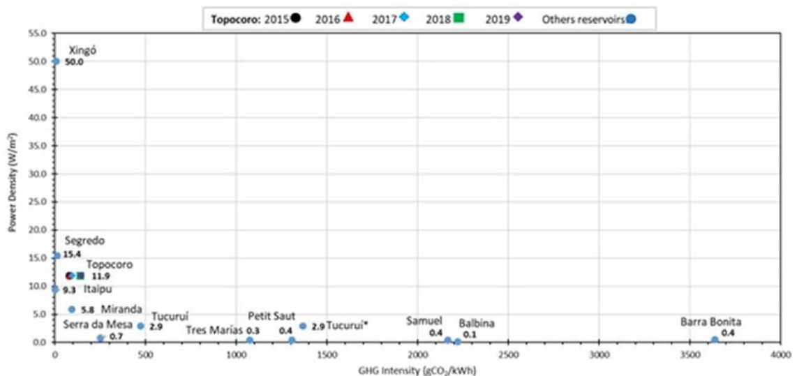
Fig. 6 | The relationship between greenhouse gas emissions intensity and power density in the tropical hydroelectric reservoir.
