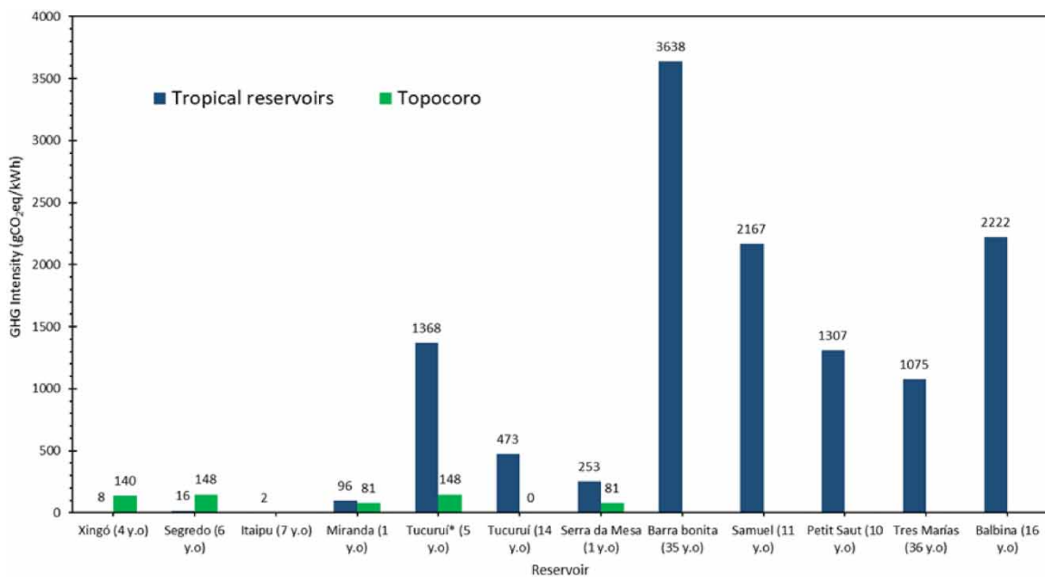
Fig. 5 | Comparison between the intensity of greenhouse gas emissions from tropical reservoirs and Topocoro. Adjusted and modified from Demarty & Bastien (2011).
