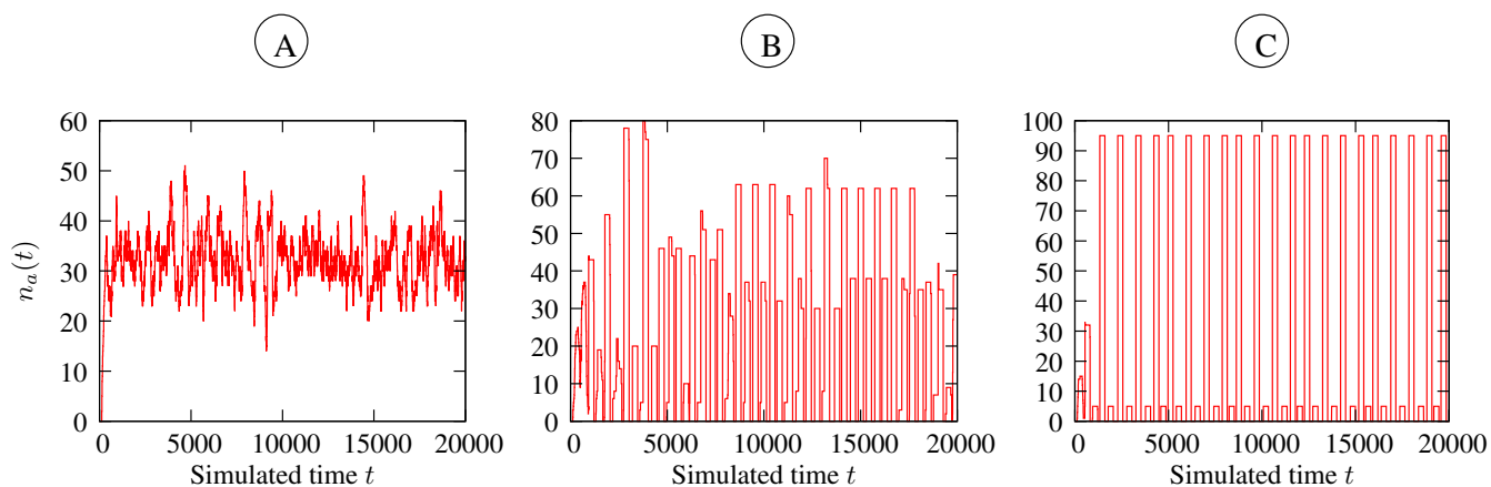
Figure 4: Three behavioral regimes emerge in the population: (A) Asynchronous, (B) Synchronous aperiodic and (C) Synchronous periodic. Each graph reports the number of active agents vs the simulated time step.
