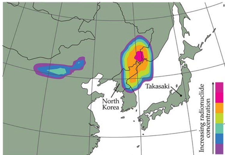
FIGURE 5. Atmospheric transport modeling (ATM) uses meteorological data to calculate how substances—for example, radionuclides—that are released into the atmosphere disperse over time and where and when they are likely to be detected. Backtracking ATM identifies where and when a release may have occurred based on the location of a detection. Shown here are the results of a backtracking calculation for an air sample containing radioactive xenon isotopes ( ^{131m}\text{Xe}/^{133}\text{Xe} ) collected at the International Monitoring System’s radionuclide station in Takasaki, Japan, on 8 April 2013. The colored regions represent the most likely areas for the isotopes’ release into the atmosphere, had it occurred one day earlier on 7 April 2013 between 03:00 and 06:00 UTC. The measured ratios of the Xe isotopes indicate that they were the product of a nuclear fission event that occurred 50 days earlier, consistent with the time of the 2013 North Korean nuclear test. (Image courtesy of the Comprehensive Nuclear-Test-Ban Treaty Organization.)
