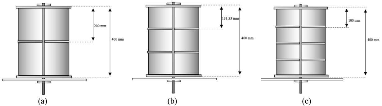
Figure 2 Savonius Wind Turbine with Fin Variation (a) Savonius geometry with variation 1 fin (b) Savonius geometry with 2 fin (c) Savonius geometry with 3 fin
