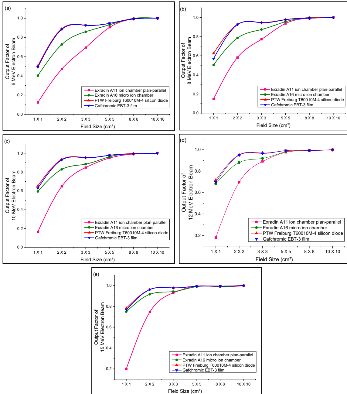
FIGURE 1. Comparison of Output factor in small field using Exradin A11 plan-parallel ion chamber, Exradin A16 micro ion chamber, PTW Freiburg T60010M-4 silicon diode, and Gafchromic® EBT-3 film
