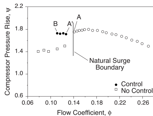
Fig. 2 Compressor pressure increase characteristic indicating time-mean operating points with and without control [13]
