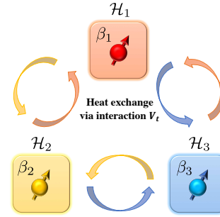
FIG. 1. Setup: We illustrate our setup with tripartite systems. The subsystem \mathcal{H}_1 , \mathcal{H}_2 and \mathcal{H}_3 are initially prepared in the Gibbs states defined by their inverse temperature and bare Hamiltonians \{\beta_1, H_1\} , \{\beta_2, H_2\} , and \{\beta_3, H_3\} . Then, at time t = 0 , we suddenly turn on the interaction V_t between the tripartite systems, which evolves under the Schrödinger's equation. Then, at time t = \tau , we suddenly turn off the interaction. The energy is pumped between the subsystems, so that we require the total energy to be conserved.
