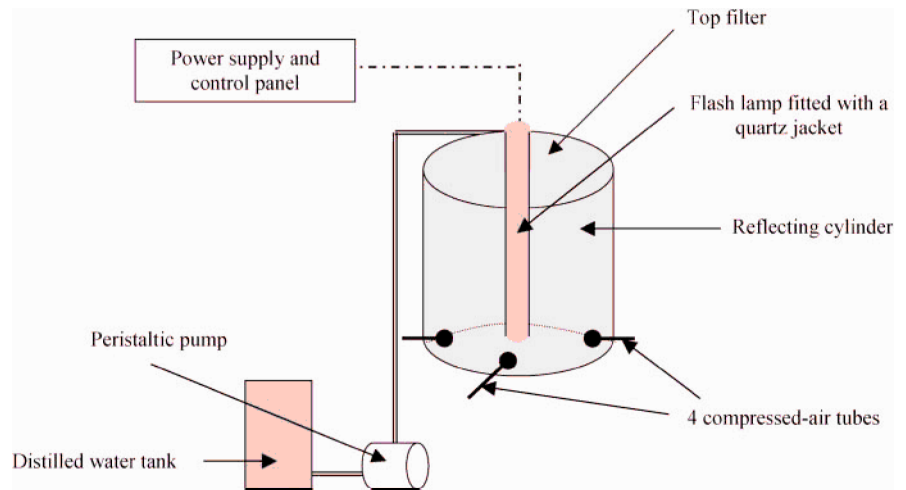
FIGURE 1. Treatment unit of One-Shot EN2/2143-1 process.
