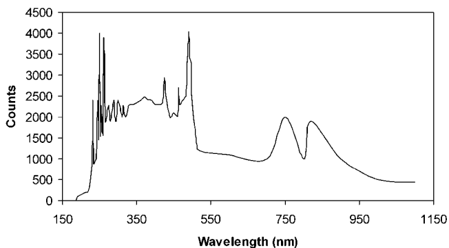
FIGURE 2. The light emission spectrum produced by the pulsed power system.
