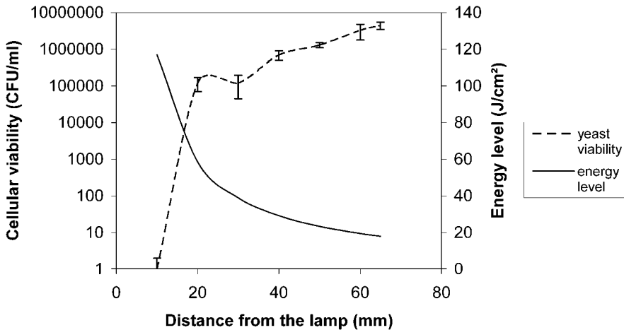
FIGURE 3. Influence of lamp distance on Saccharomyces cerevisiae viability after 24 pulses at 551 J. Vertical bars correspond to confidence intervals at the 95% level.
