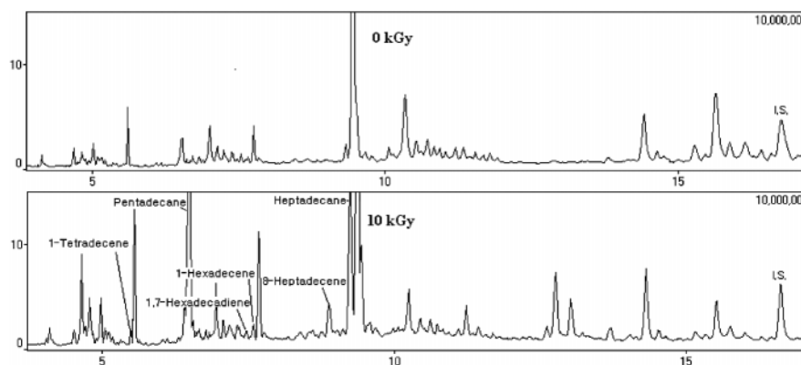
FIGURE 1. Chromatograms for the hydrocarbons from nonirradiated and irradiated (10 kGy) dried squids.
