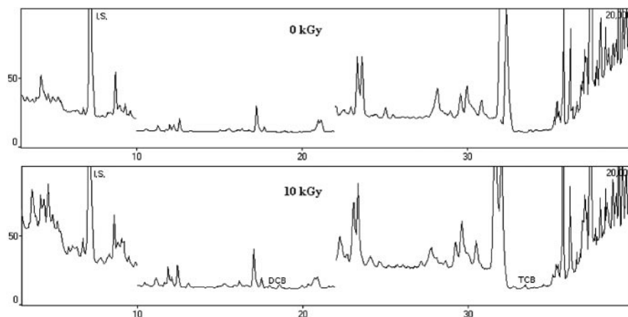
FIGURE 2. Chromatograms of 2-alkylcyclobutanones from nonirradiated and irradiated (10 kGy) dried squids. DCB, 2-dodecylcyclobutanone; TCB, 2-tetradecylcyclobutanone.
