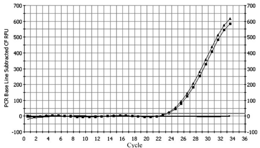
FIGURE 2. Real-time PCR amplification of 18S rRNA gene fragment with the mold-specific primer-probe set. ■, Byssoschlamys fulva ATCC 24474; ▲, Penicillium digitatum ATCC 10030. Alicyclobacillus acidocaldarius ATCC 43030, Escherichia coli DH-5 \alpha , Lactococcus lactis 2301, Listeria monocytogenes V7, Pseudomonas putida 49451, grape, orange, and apple gave no response (horizontal line). CF RFU, curve fit relative fluorescence units.
