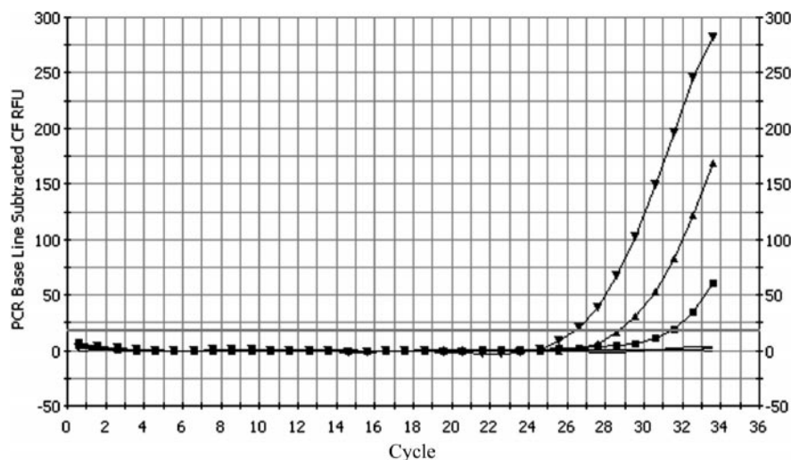
FIGURE 3. Sensitivity of detection for real-time PCR product obtained with the environmental mold KW01 diluted in orange juice. ▼, 4.3 \times 10^2 CFU per reaction; ▲, 4.3 \times 10^1 CFU per reaction; ■, 4.3 CFU per reaction. The uninoculated orange juice (blank control) gave no response (horizontal line). CF RFU, curve fit relative fluorescence units.
