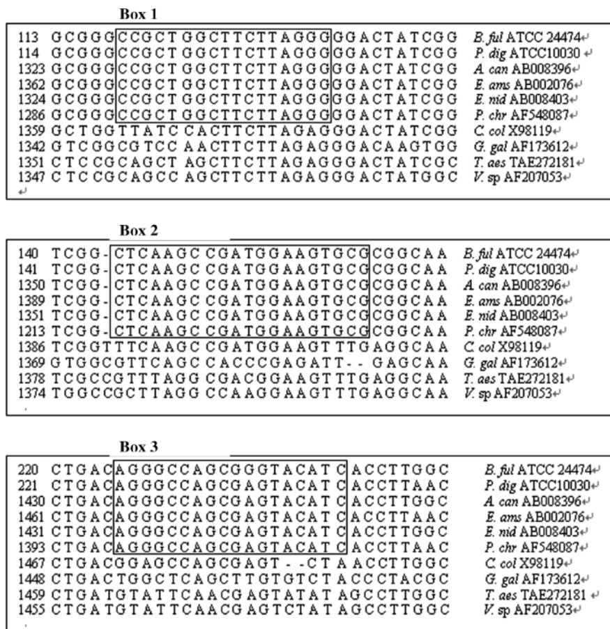
FIGURE 1. Alignment of 18S rRNA gene fragments from Byssoschlamys fulva ( B. ful ) ATCC 24474, Penicillium digitatum ( P. dig ) ATCC 10030, Aspergillus candidus ( A. can ) AB008396, Eurotium amstelodami ( E. ams ) AB002076, Emericella nidulans ( E. nid ) AB008403, Candida colliculosa ( C. col ) X98119, Gallus gallus ( G. gal ) AF173612, Triticum aestivum ( T. aes ) TAE272181, and Vitis sp. ( V. sp. ) Soltis and Soltis 2519 AF207053. Boxed nucleotide sequences were used to design PCR primers and probe. Box 1 refers to the primer MoldFP; box 2 refers to the probe MoldTP; and box 3 refers to the complement reverse fragment of primer MoldRP.
