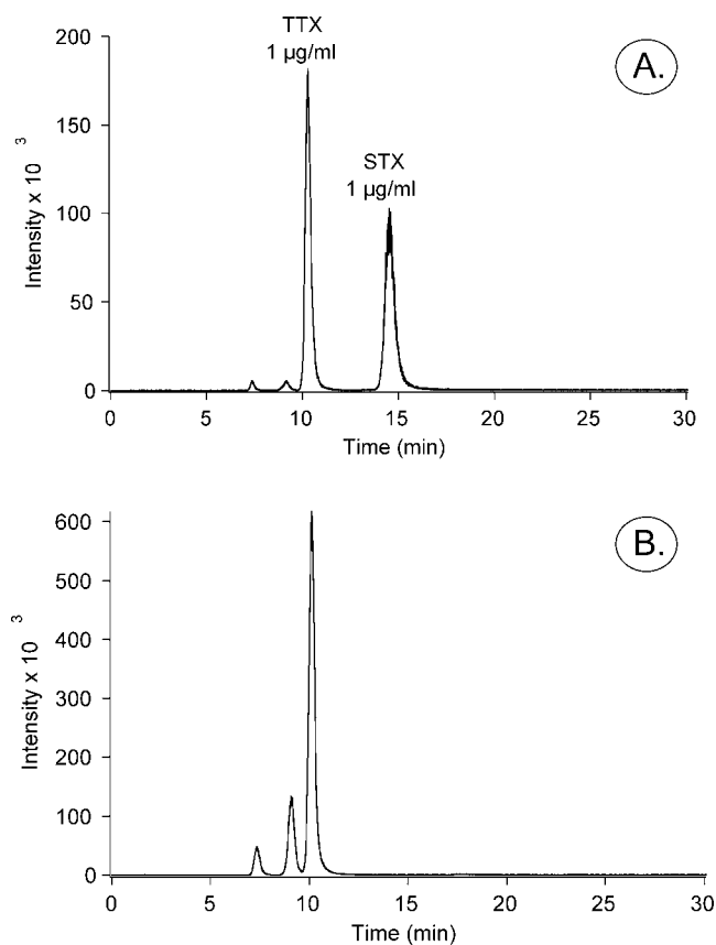
FIGURE 1. Electrospray-ionization multiple-reactions monitoring mass spectrometry (LC/ESI/MS) chromatograms representing the selected ion transitions for tetrodotoxin (TTX) [ M + H ] + at m/z 320 fragmenting to ions at m/z 302, 256, and 162 and saxitoxin (STX) [ M + H ] + at m/z 300 fragmenting to ions at m/z 282, 204, and 179 for a 1- \mu\text{g}/\text{ml} (each) mixed standard of TTX and STX (A) and a representative subsample (fish 1 from Table 1) of fish muscle from the implicated lot of suspect puffer fish collected from the California supplier (B).
