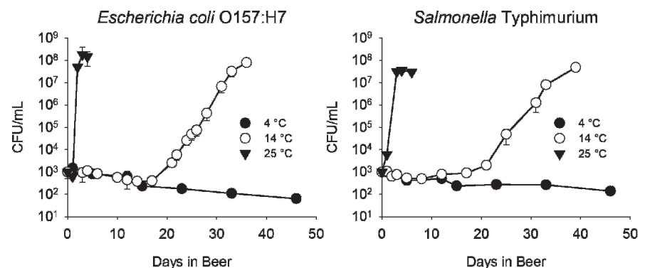
FIGURE 3. Effects of storage temperature on the survival of E. coli O157:H7 and Salmonella Typhimurium in alcohol-free beer. Data points are the means of triplicate flasks; error bars are \pm standard deviations.
