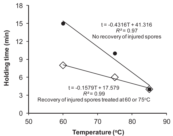
FIGURE 4. Process time required to inactivate Bacillus cereus ATCC 9818 spores in rice to below the detection limit of 10 CFU/g ( \geq 7.0 -log reduction) at 600 MPa and various process temperatures (T), with recovery of injured spores during subsequent storage of samples at 25°C ( \diamond ), or without recovery of injured spores (i.e., viable spores were below 0.48 log MPN/g) during storage at 25°C ( \bullet ).
