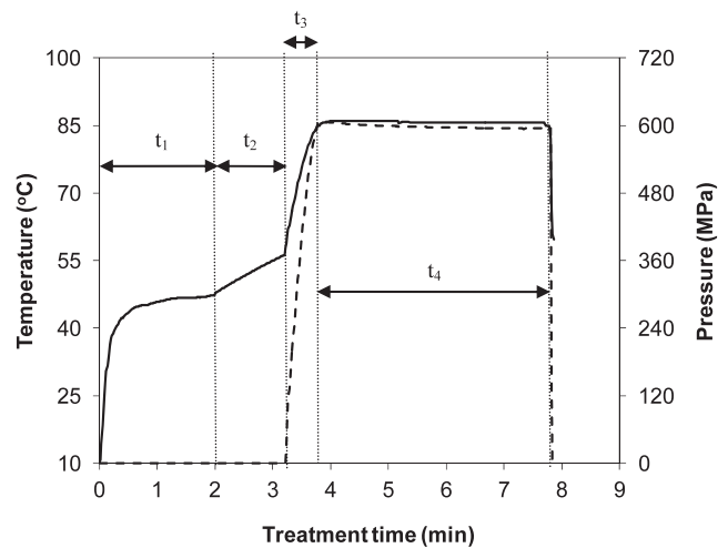
FIGURE 1. Representative pressure and temperature histories of rice samples during pressure-heat treatment (600 MPa and 85°C) for 4 min. t_1 , preheating time in a water bath (47°C); t_2 , preheating time inside the pressure chamber; t_3 , pressure come-up time; t_4 , pressure holding time. The dashed and solid lines represent pressure and temperature changes, respectively.
