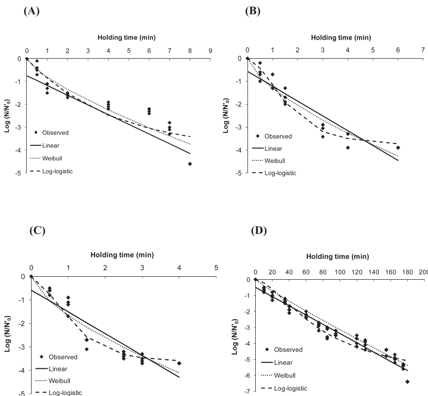
FIGURE 2. Inactivation kinetics of Bacillus cereus ATCC 9818 spores in rice during treatment at 600 MPa and various process temperatures: 60°C (A), 75°C (B), 85°C (C), or 0.1 MPa and 85°C (D), fitted by linear, Weibull, and log-logistic models. N 0 and N are the spore counts (in CFU per gram) immediately after come-up time and after holding time, respectively. The spores were inoculated into the product at an inoculum level of 1.1 × 10 8 CFU/g prior to treatments. Detection limit was 10 CFU/g.
