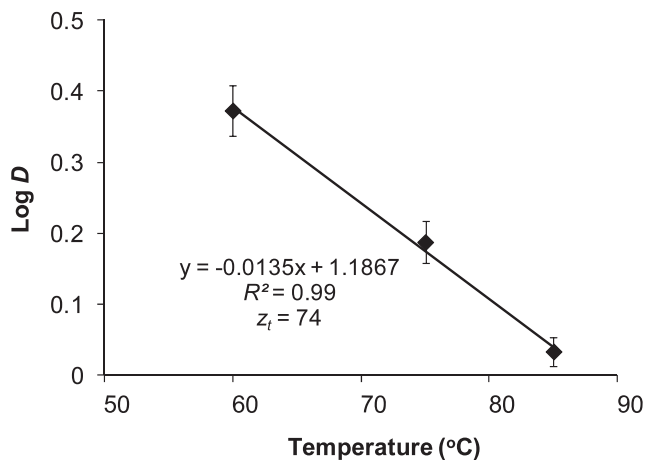
FIGURE 3. Estimation of z_T -value of Bacillus cereus ATCC 9818 spore inactivation in rice by combined pressure-heat treatment (600 MPa, 60 to 85°C).
