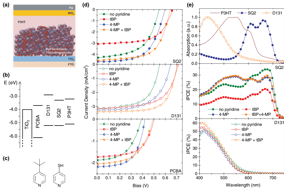
FIG. 1. (a) Schematic of the solar cell geometry used in this study. (b) Energy diagram of \text{TiO}_2 , PCBA, D131, SQ2, and P3HT. Energy levels from Refs. 2, 3, 8, and 16. (c) Chemical structures of the two pyridines tBP (left) and 4-MP (right) used as interfacial modifiers. (d) Current density-voltage curves for solar cells with different pyridine configurations and the dyes SQ2, D131, and PCBA (from top to bottom). (e) Typical absorption spectra of P3HT on glass and \text{TiO}_2 nanoparticle films sensitized with SQ2 and D131 (top), and IPCE spectra of solar cells with different pyridine configuration with SQ2 and D131 as sensitizer.
