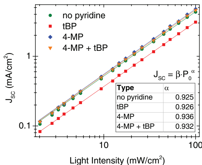
FIG. 3. J_{sc} as a function of incident light intensity for SQ2 solar cells with different pyridine configurations. Lines represent results from power law fits.
