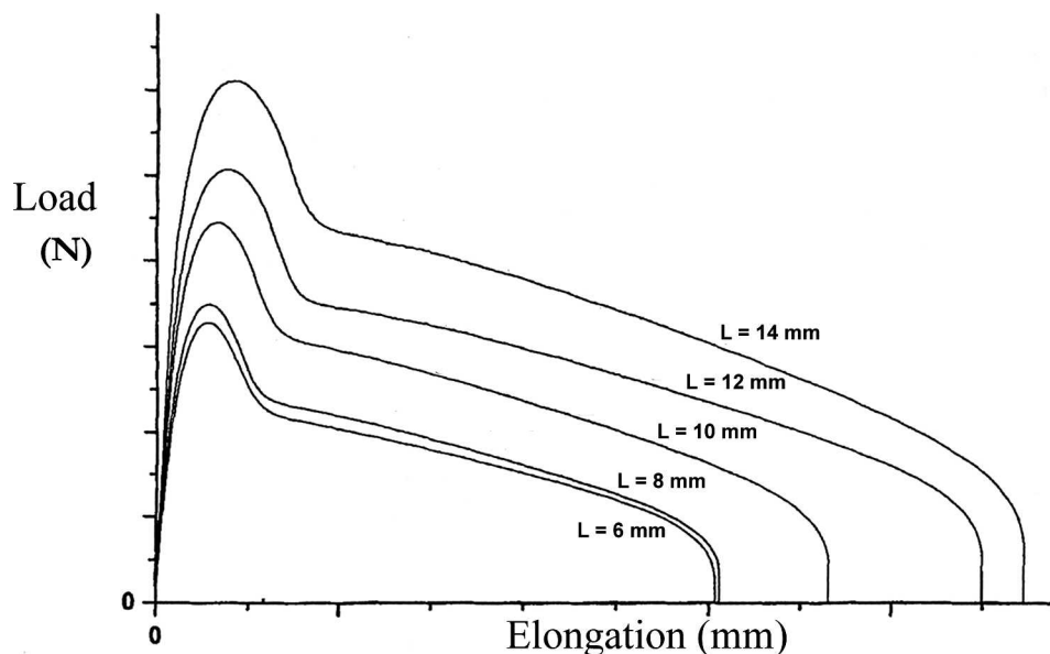
Figure 2. Load-elongation curves for a range of ligament lengths ( L_s ). The second requirement for essential work of fracture (EWF) test validity: curves must appear similar in shape.
