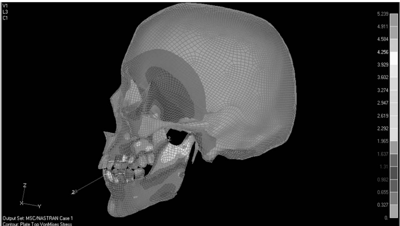
Figure 5. Pattern of von Mises stress distribution (in MPa).
