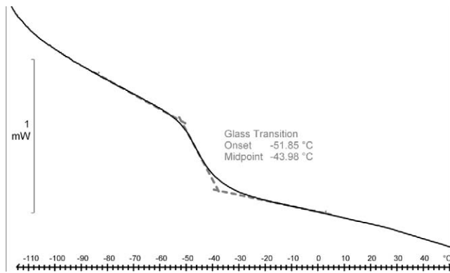
Figure 4. Representative differential scanning calorimetry (DSC) thermogram for a ligature illustrating the glass transition. The glass transition temperature ( T_g ) is given as the midpoint of a line connecting the two baselines (dotted lines drawn with the DSC software program).
