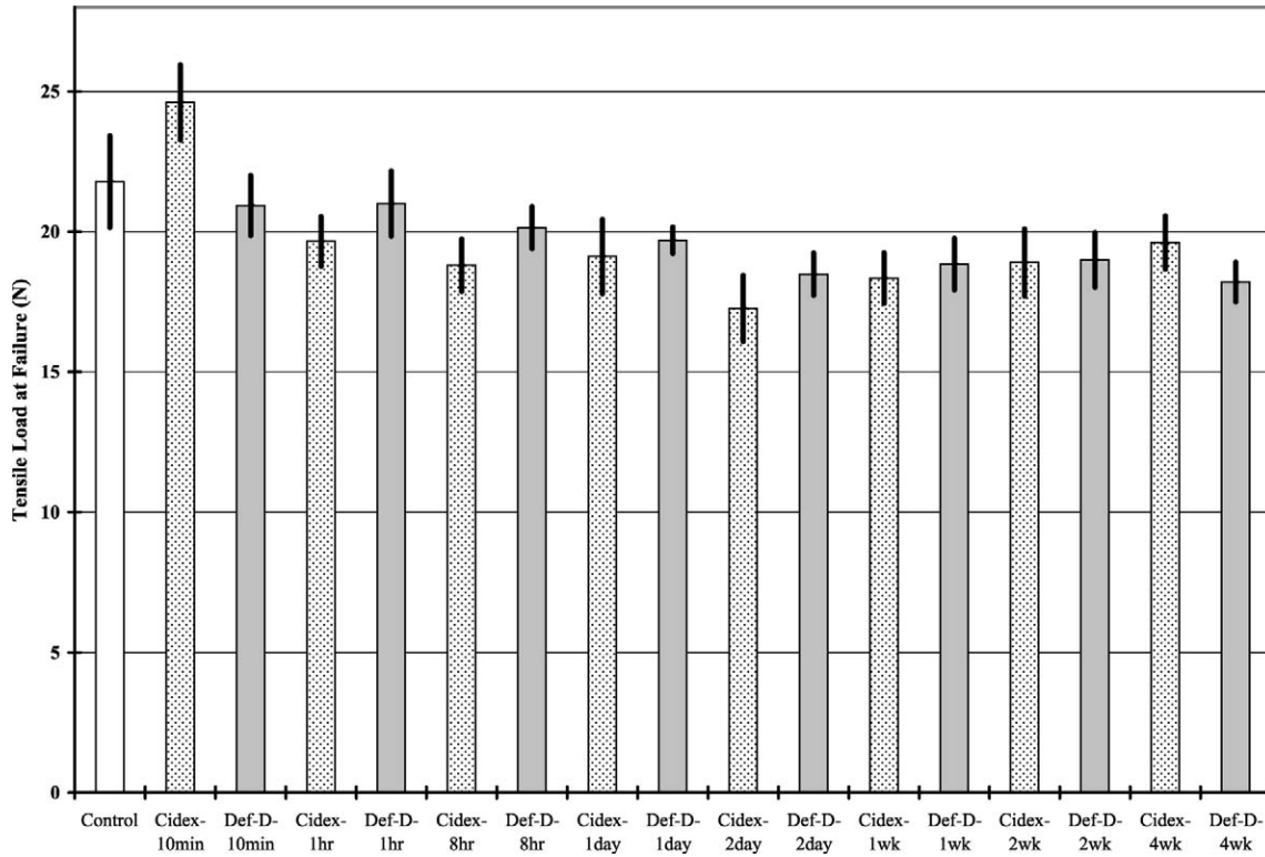
Figure 2. Tensile load at failure of ligatures from 3M Unitek exposed to Cidexplus and Vital Defense-D. The error bars represent standard deviation.
